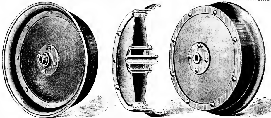
Figs. 5632-5634. KALAMAZOO ALL-STEEL HAND-CAR WHEEL. Malleable-iron Flanged Hub, Double Steel-plate Center, Wood Felloe, Re-enforced with Steel Rings.
